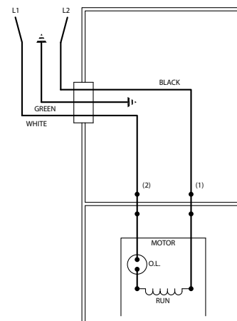
WIRING DIAGRAM FOR MODELS "N55", "N55-A", "N55-B", "N55-C" 9/82 (VN) thru Current
